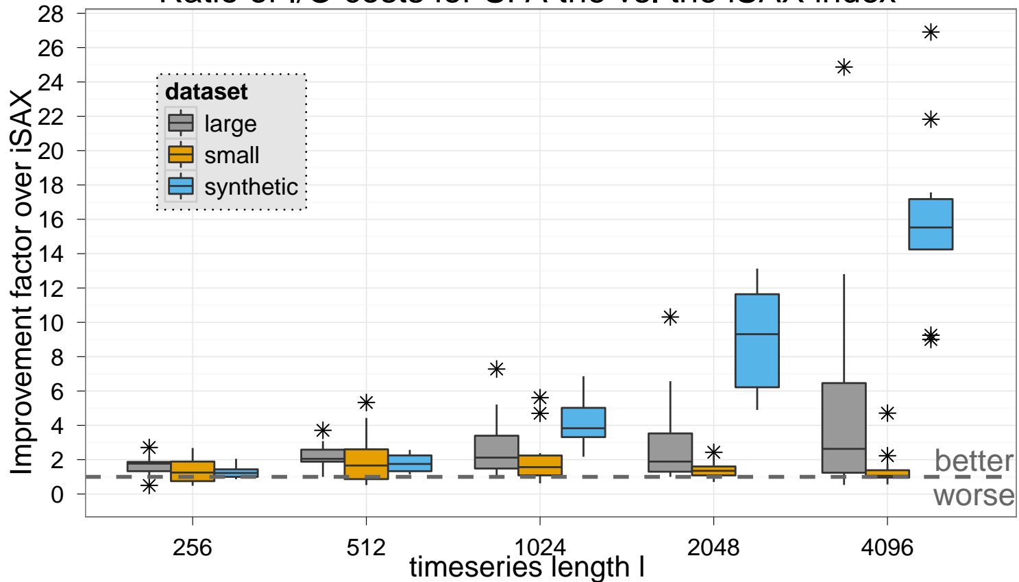
Ratio of I/O costs for SFA trie vs. the iSAX index
