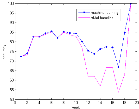
Figure 4: SVM classification accuracies per week. The baseline accuracy is computed as \min(p_i, 1 - p_i) , where p_i denotes the weekwise dropout probability.
