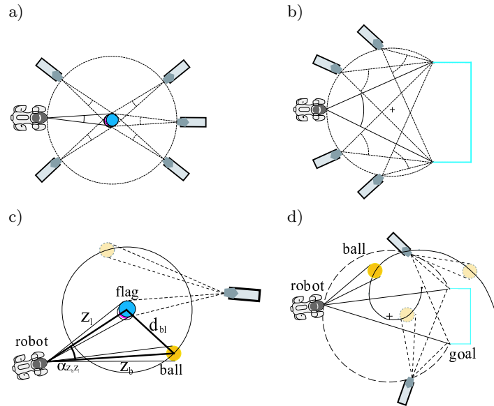
Fig. 1. Single percept: a, b) When a flag or a goal is seen, the robot can calculate its distance to it, but not its exact position, a circle remains for all possible robot positions
