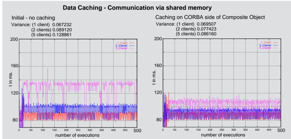
Figure 3-9: Minimizing Data Accesses: Effects of Caching
