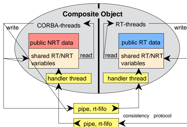
Figure 2-2: Consistency Protocol and Communication Inside a Composite Object
