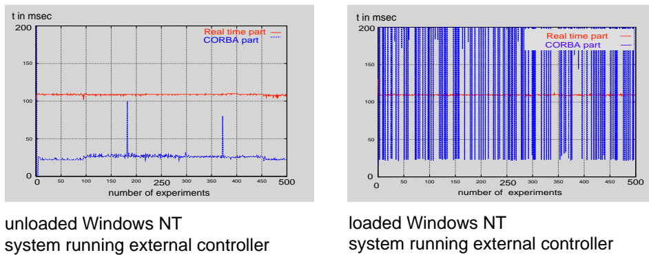
Figure 3-4: Execution of Java Controller Versus Simulation's Period
