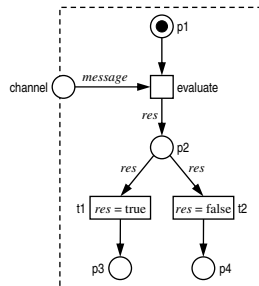
Fig. 1. A high-level oWFN.
