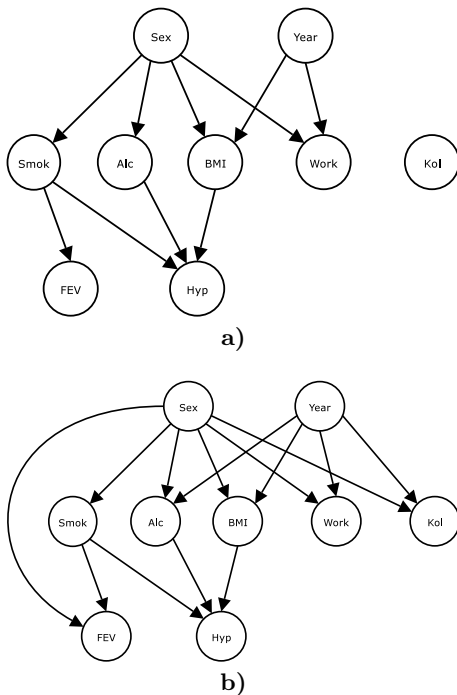
Figure 4: Network structure for the KSL dataset constructed by the authors
